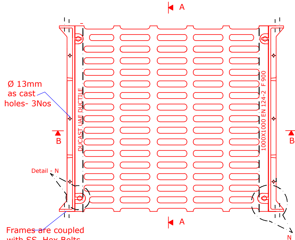
Plan View of Grating
