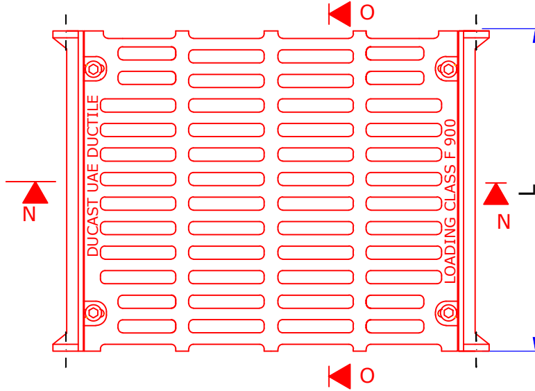
PLAN VIEW
