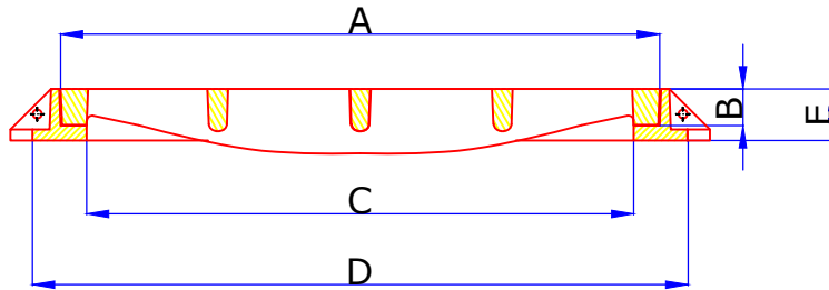
SECTIONAL VIEW @ N-N
