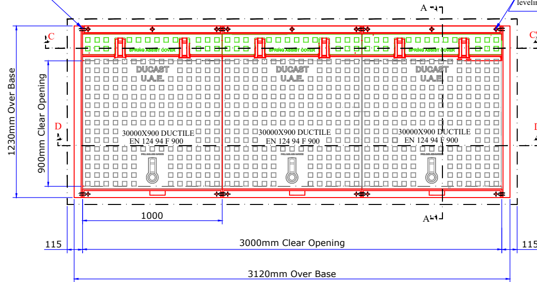
Plan view of cover & frame
