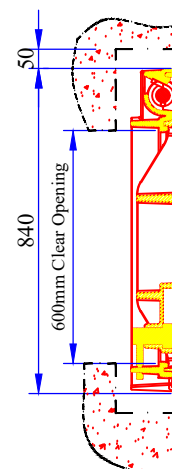
SECTION C-C
