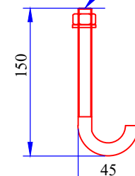
J-Bolt Details
