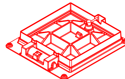
ISO METRIC VIEW (COVER REAR )
