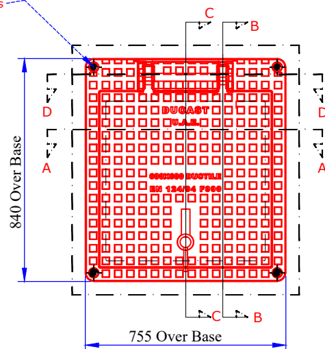
PLAN VIEW OF COVER & FRAME
