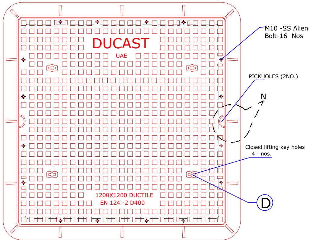
Plan View of Cover & Frame
