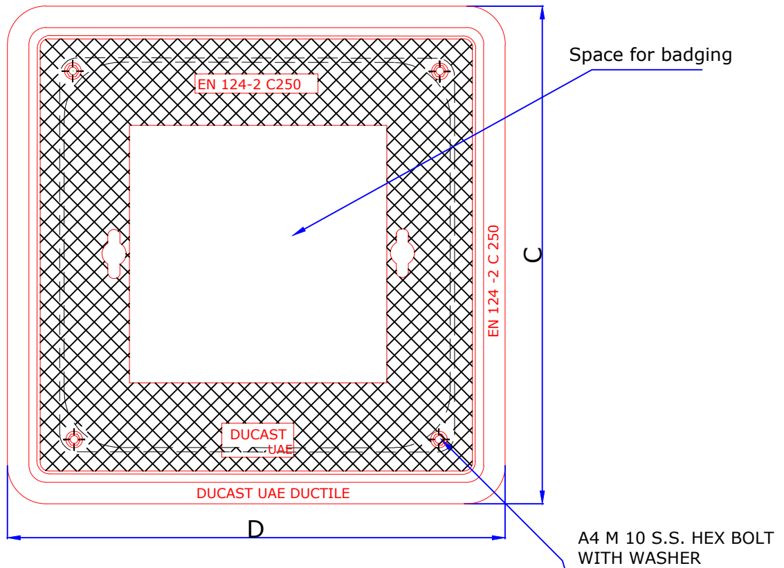
PLAN OF COVER & FRAME
