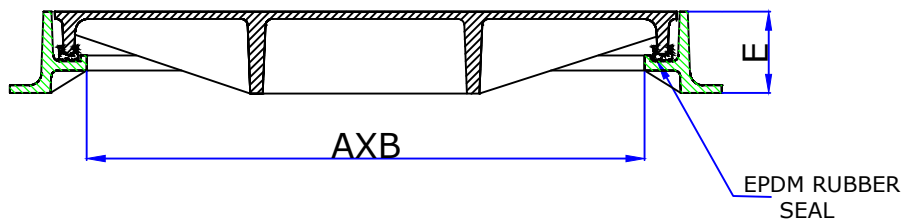
SECTIONAL VIEW OF COVER & FRAME
