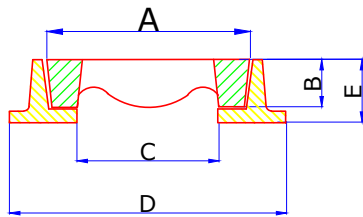
SECTIONAL VIEW
