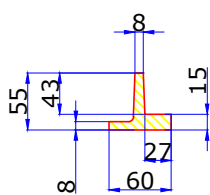
Section-HH
