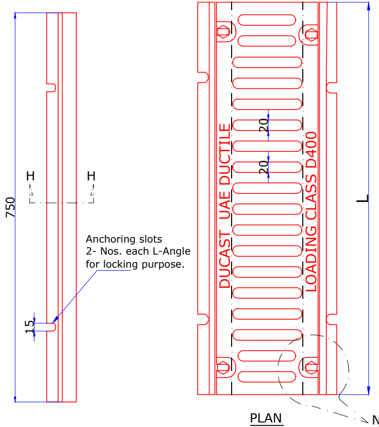
L-Angle Details
