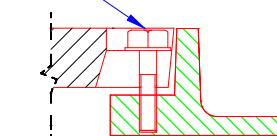
SECTION M-M
